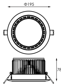
CUT-OUT:Φ175MM
