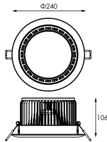
CUT-OUT: Φ210MM
