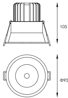
CUT-OUT:Φ85MM
