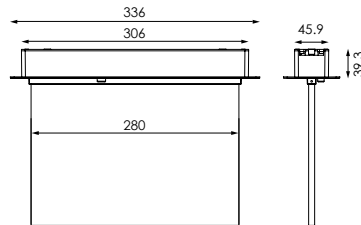
CUT-OUT:312*51MM
